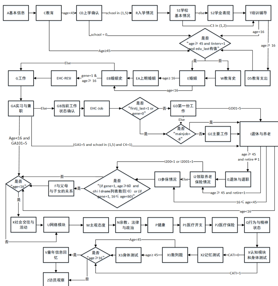
图 1. CFPS2020 个人问卷模块间跳转逻辑
